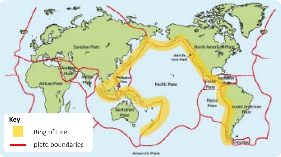
Earth’s tectonic plates
